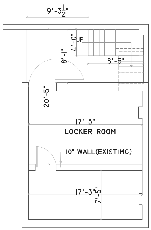
BASEMENT FLOOR (EXISTING)
