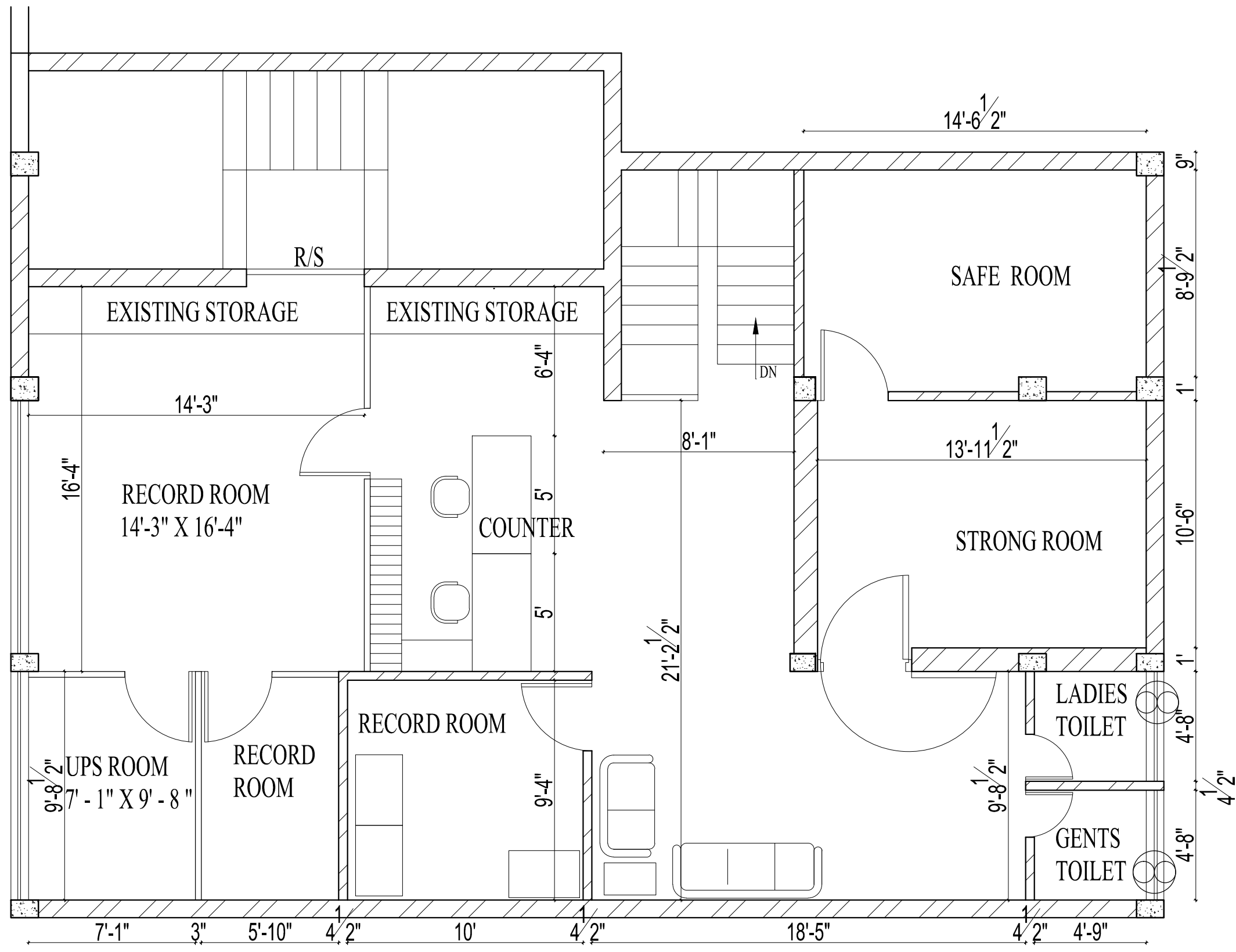
PROPOSED FIRST FLOOR OPTION - I
