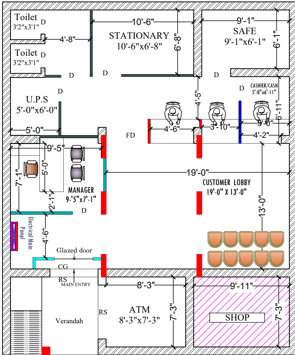
ROAD GROUND FLOOR PLAN
