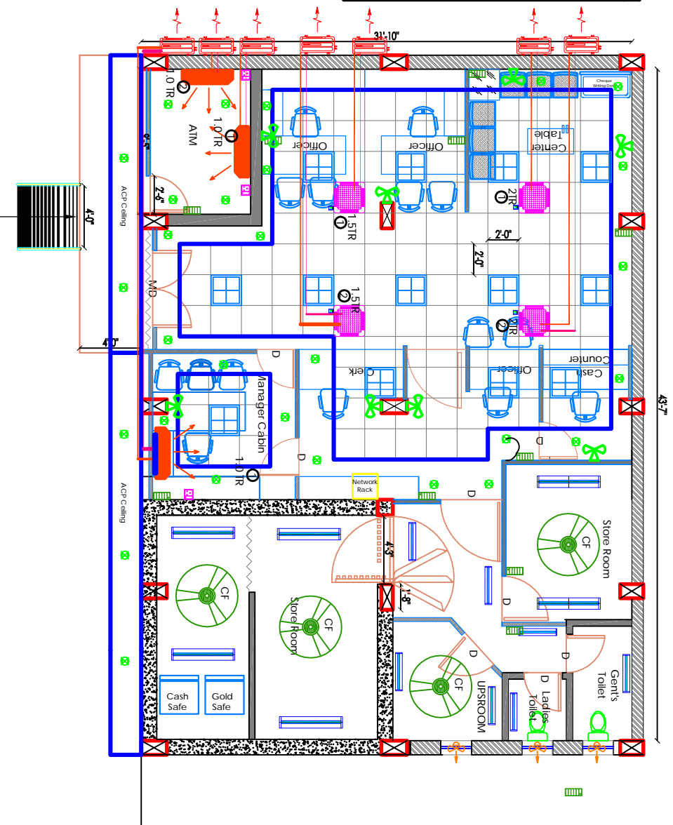
ELECTRICAL LAYOUT PLAN
