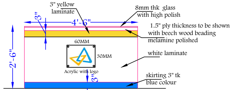
FRONT ELEVATION
