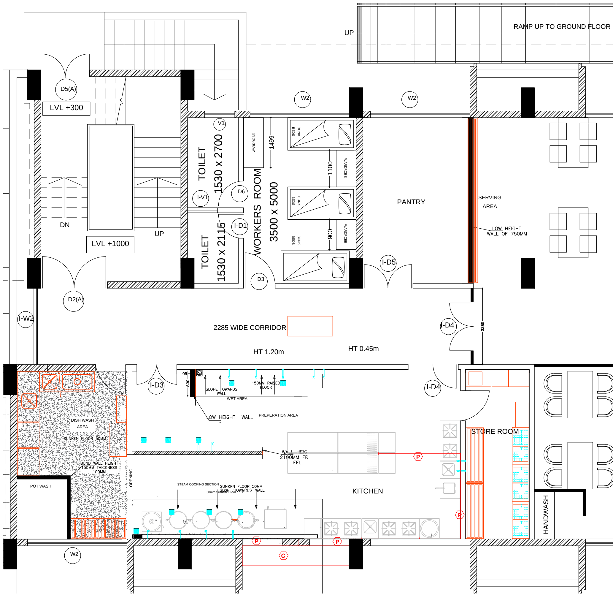
L.P. GAS PIPELINE LAYOUT
