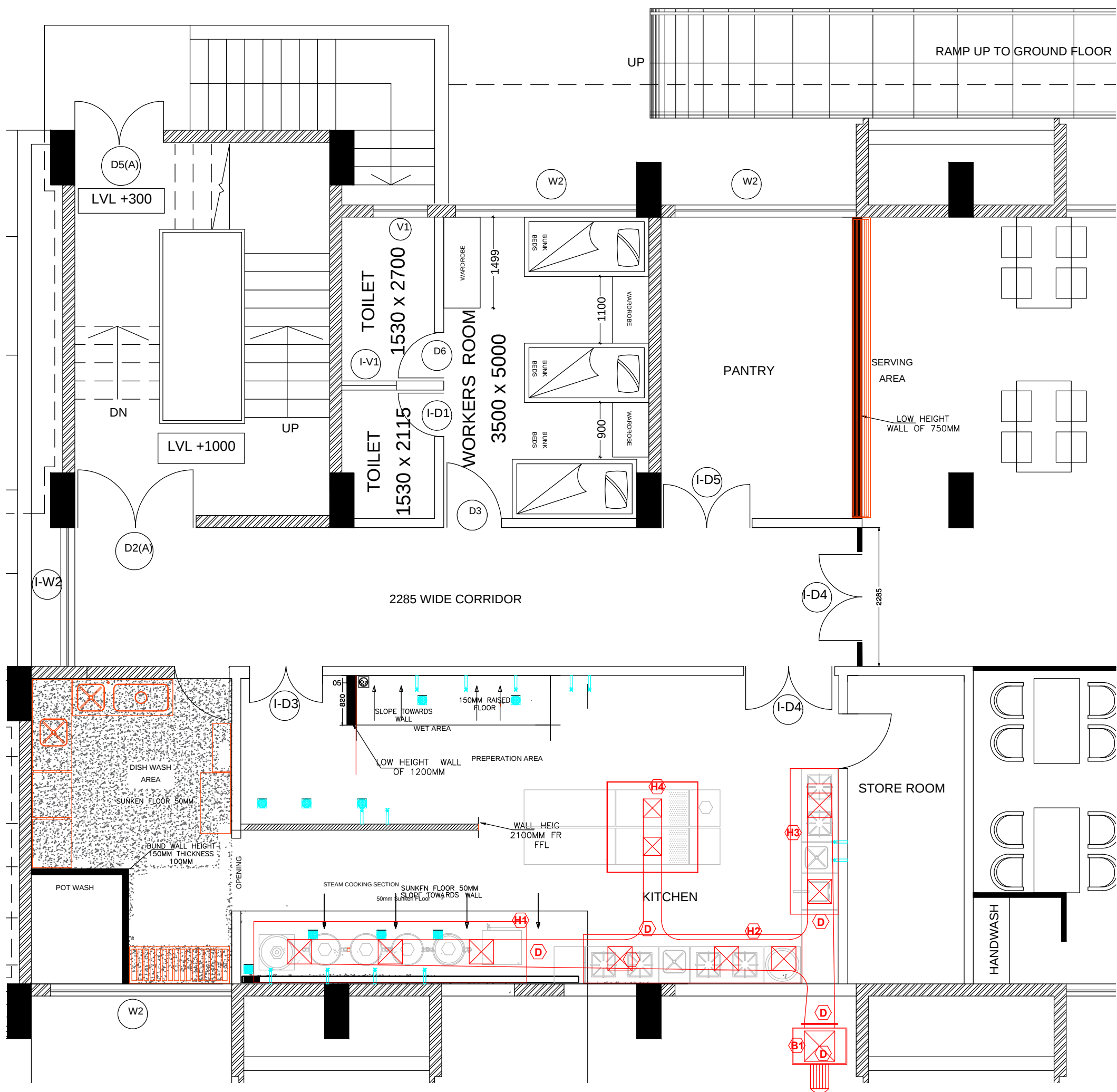
VENTILATION SYSTEM LAYOUT
