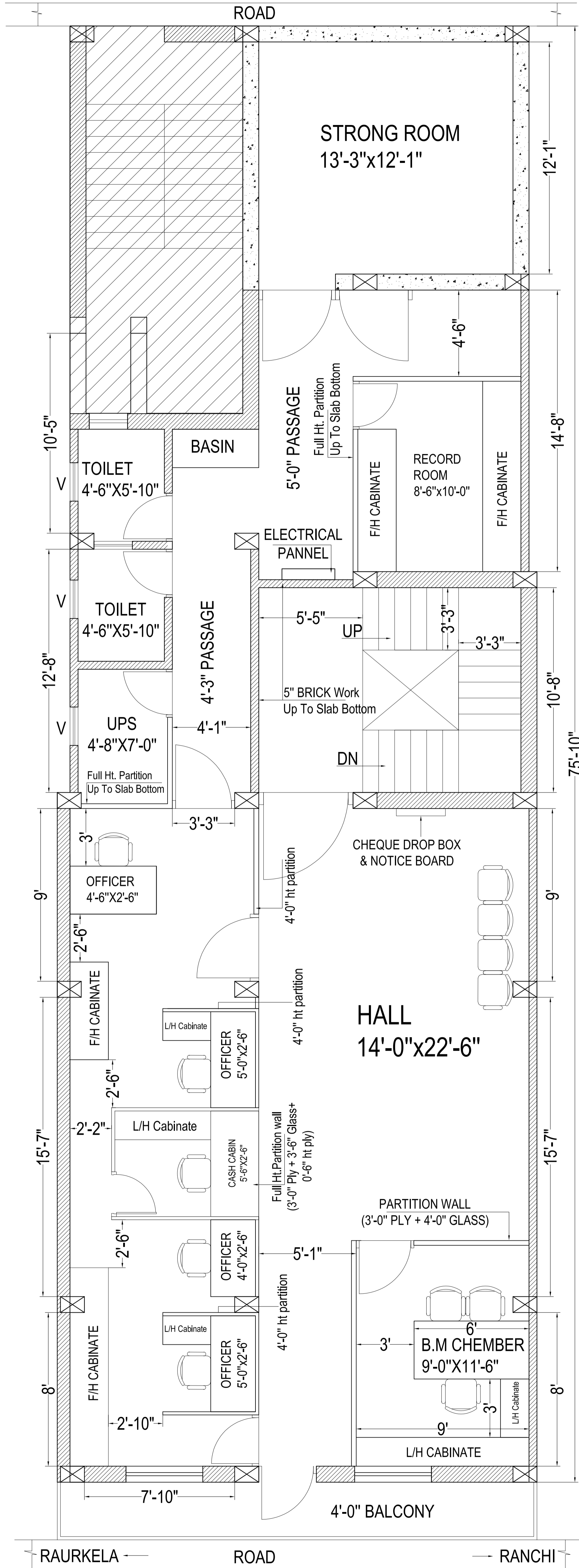
FIRST FLOOR PLAN AREA = 1451.06 SQ FT.
