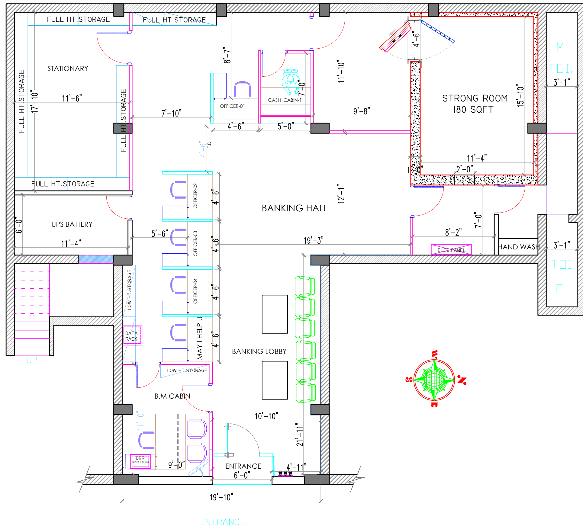
BARKAGAON BRANCH CARPET AREA-1650 SQFT Internal
